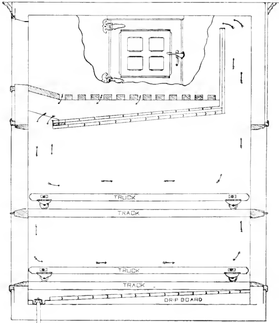
FIG. 8.—Cross-section.
